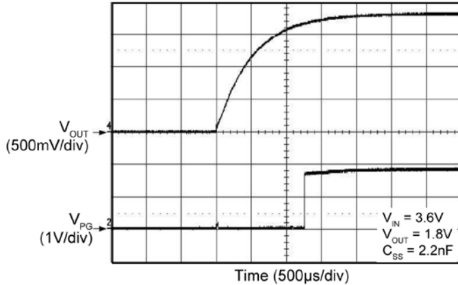
Start-Up PGOOD
